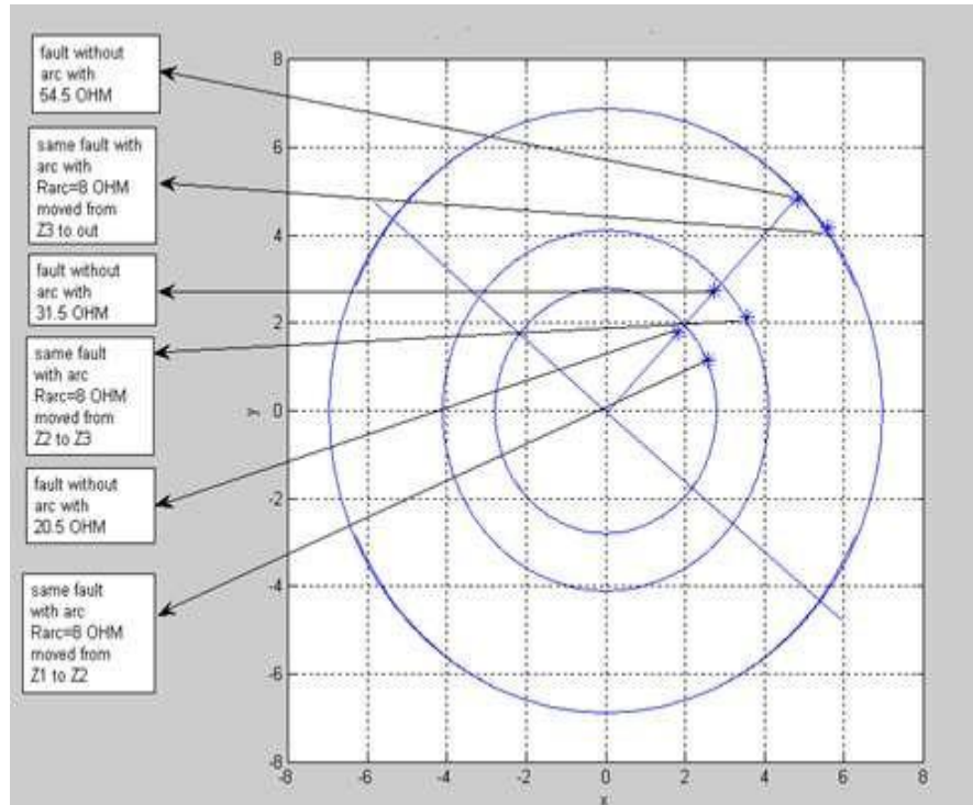
Figure 9 Impedance characteristic
