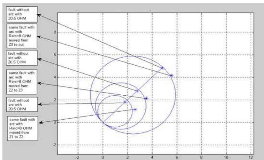
Figure 10 mho characteristic
