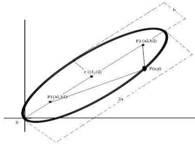
Figure 3 Ellipse
