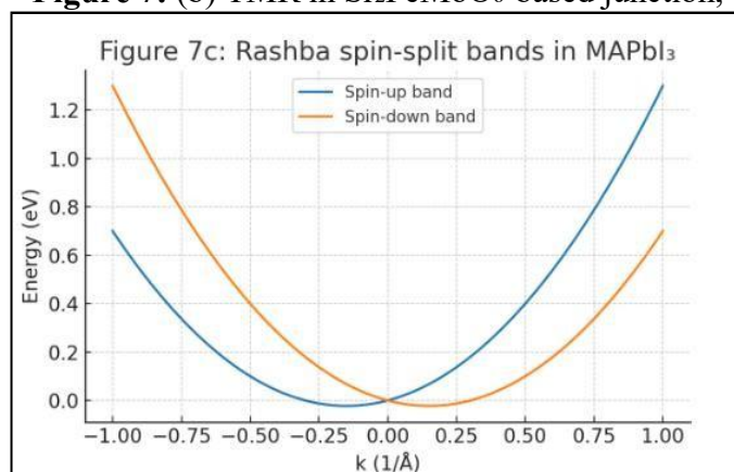
Figure 7: (c) Rashba spin-split band structure in MAPbI 3 .
