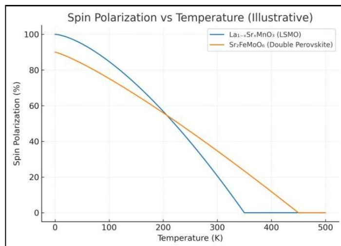
Figure 3: (LSMO shows nearly 100% polarization at low T, Sr 2 FeMoO 6 maintains high values at room T)
