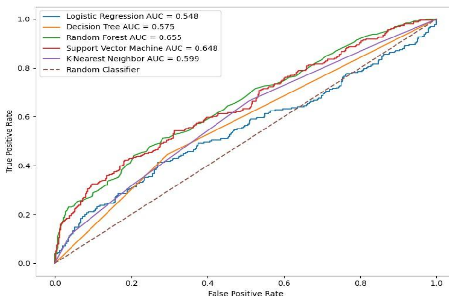
Figure 3. ROC Curve Comparison
