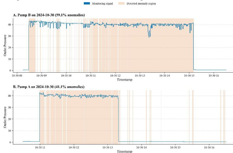
Figure 3. Time-series operating regimes with detected anomalous intervals: (A) Pump B on 30 October 2024; (B) Pump A on 30 October 2024
