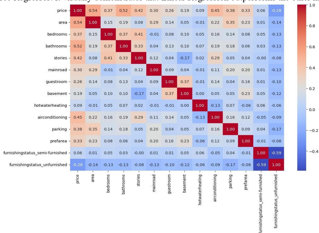
Figure 3: Correlation Heatmap of Housing Dataset
