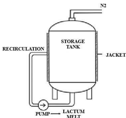
Figure 2: Storage Tank
