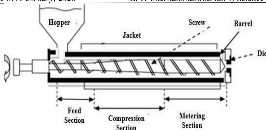
Figure 5: Extruder Arrangement [80]
