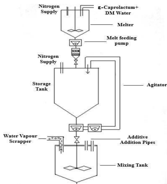
Figure 1: Lactam Preparation Process (Pre-Polymerization Process).
