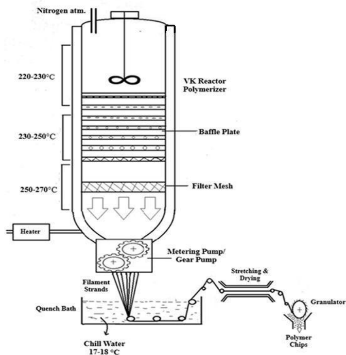
Figure 3: VK reactor – Polymerization assembly of Nylon 6.
