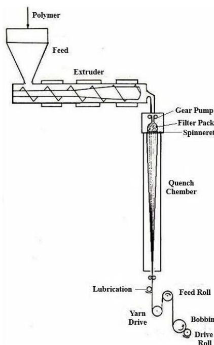
Fig. 7 Melt spinning. [83]
