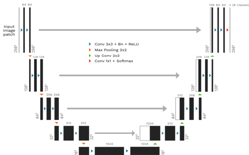
Figure III. U-Net Architecture
