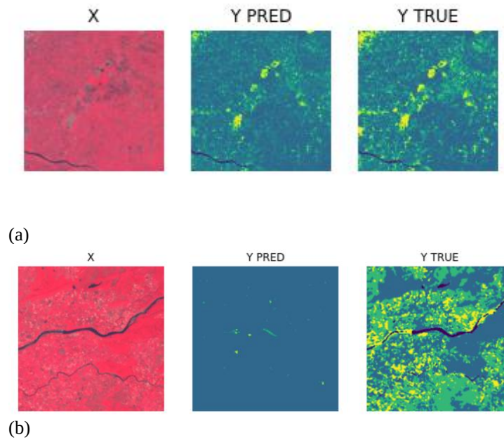
Figure V. Experiment result
