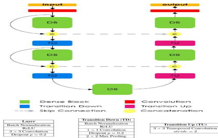
Figure IV. Tiramisu Architecture [23]
