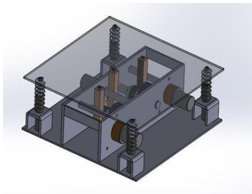
Fig.9- Perspective View
