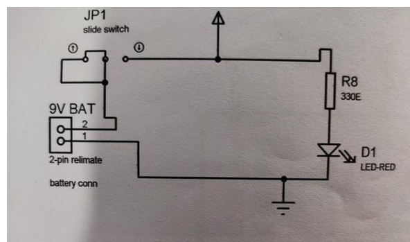
Fig.3- Circuit 2
