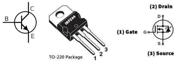
Fig.29-IRFZ44
