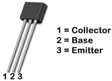
Fig.28-BC547
