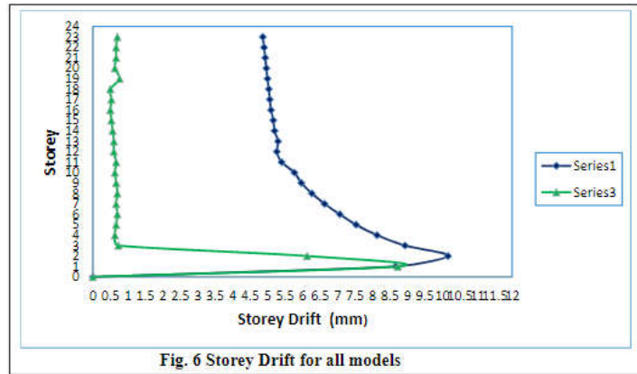
Fig. 6 Storey Drift for all models
