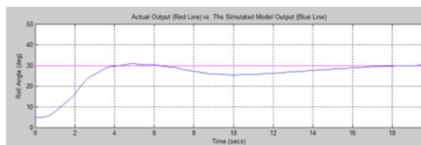
Figure 4.12 Response Simulation Test Roll Actual and Estimated current system Heading 30 0 and Wave Interference Sea State 6
