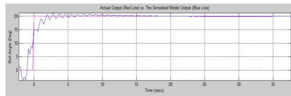
Figure 4.3 Roll Response Simulation Test System Actual and Estimated time Heading 20^{\circ} and Disturbance Wave Sea State 6
