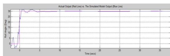
Figure 4.5 Response Roll Simulation Test System Actual and Estimated time Heading 30^{\circ} and Without Disturbance
