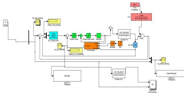
Figure 4.1 Diagram Stability Rolling Simulation by Wave Interference Sea State 6 with linear dynamics modeling ship
