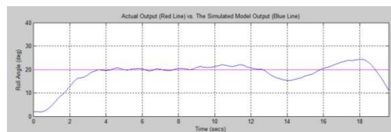
Figure 4.11 Response Simulation Test Roll Actual and Estimated time Heading System 200 and Disturbance Wave Sea State 6
