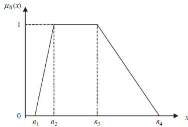
Figure 4:- A Trapezoidal Fuzzy number
