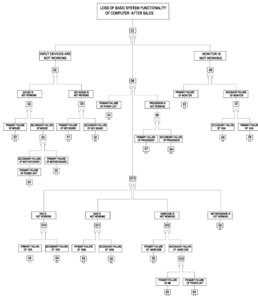
FIGURE 1-FAULT TREE OF THE PERSONAL COMPUTER SYSTE
