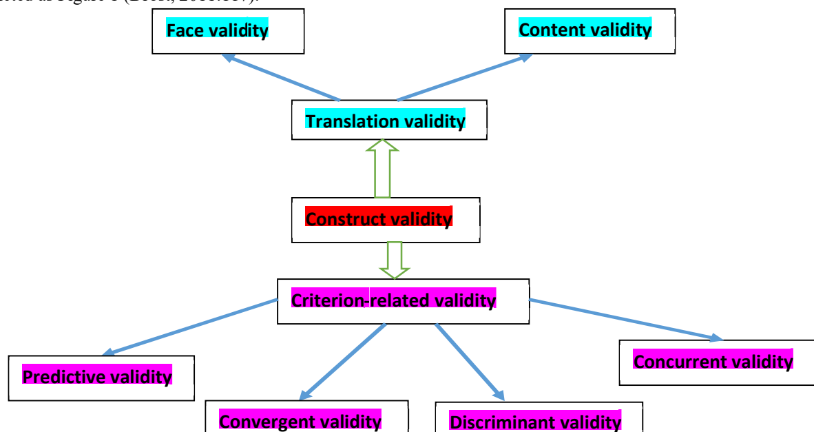
Figure 1: Types of Construct Validity.
