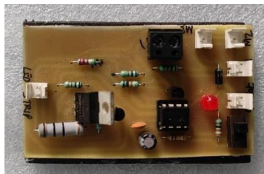
Fig.6-Inverter Layout
