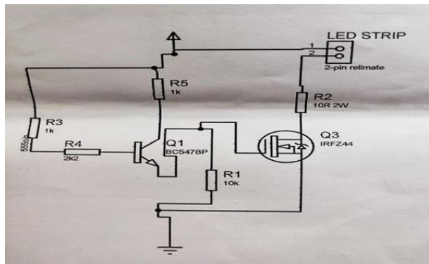
Fig.2- Circuit 1
