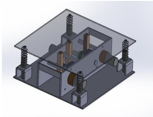
Fig.9- Perspective View
