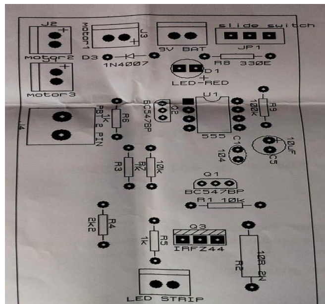
Fig.5- Component Layout
