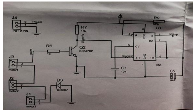
Fig.4- Circuit 3
