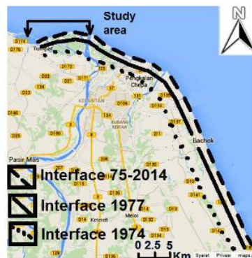
Fig.17. Variation of freshwater/saltwater interface on the first coastal aquifer of Tumpat, Kelantan during the period from (1974-2014) Source: Updated after [2].
