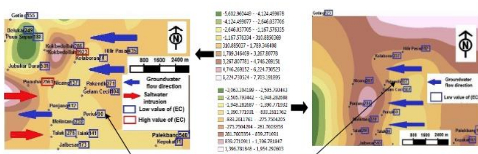
Fig.14. Distribution of the (EC) values ( \mu\text{s}/\text{cm} ) during the wet season in the first aquifer of
