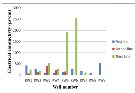
Fig.5. Variation of electrical conductivity in the wells during the dry season in the first aquifer of Tumpat
