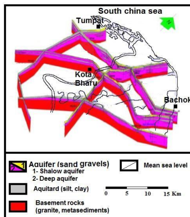
Fig.3 Cross section of Tumpat, Kelantan
