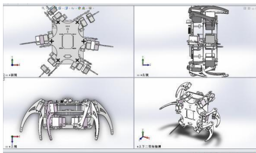
Figure 4 SolidWorks simulation
