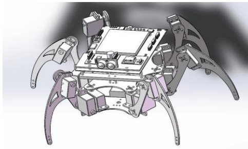
Figure 1 SolidWorks Simulation
