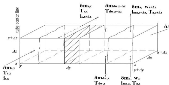
Figure 3: The elementary control volume of the delugeable horizontal bare flat tube bundle
