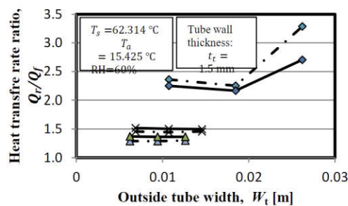
Figure 7: Effect of the tube height on the heat transfer rate ratio of round and flat tube bundle
