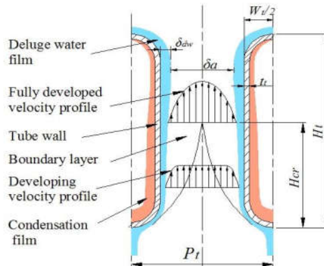
Figure 4: Tube bundle section, illustrating the air-side flow between two adjacent tubes The output data which obtained by different methods of analysis are shown in Table 1.
