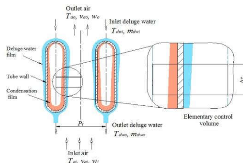
Figure 2: Schematic diagram of two adjacent tubes in a delugeable flat bare tube bundle
