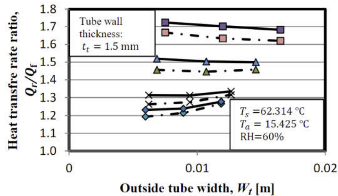
Figure 5: Effect of the tube pitch on the heat transfer rate ratio of round and flat tube bundle
