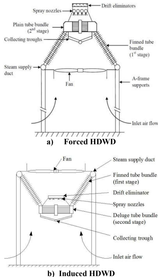
Figure 1: Schematic diagram of the HDWD
