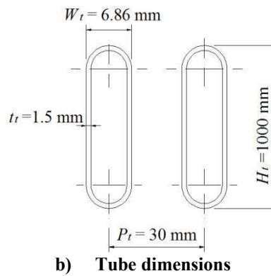
Figure 9: Tube bundle layout and dimensions
