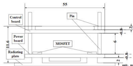
Figure 6 drive structure
