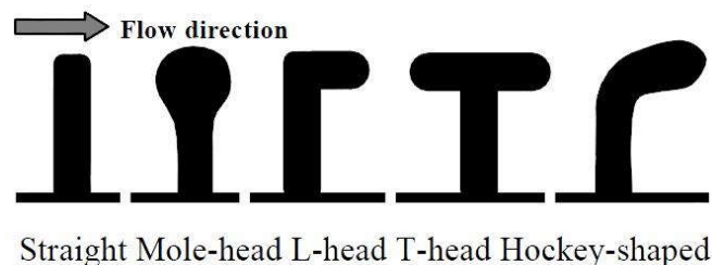
Fig 1. Types of Dike Shapes in Plan.
