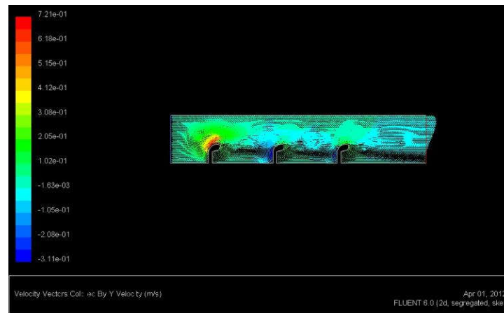
Fig 7. The velocity vectors in Y direction around Consecutive Hockey-shaped Spur Dike
