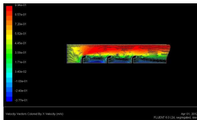
Fig 6. The velocity vectors in X direction around Consecutive Hockey-shaped Spur Dike
